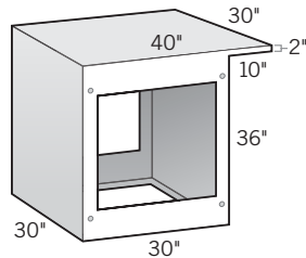
Cabinet w/10" Cantilever Backside 30"D x 30"L x 36"H OLPLSCHBS
