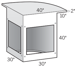
BAR-HEIGHT 90° Radius Corner Cabinet w/10" Cantilever 30"D × 30"L × 40"H OLPLSBHRC
