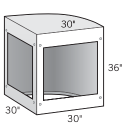
90° Radius Corner Cabinet 30"D × 30"L × 36"H OLPLSOCHR
