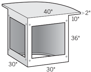
90° Radius Corner Cabinet w/10" Cantilever 30"D × 30"L × 36"H OLPLSCHRC
