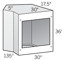
135° Radius Corner Cabinet 30"D × 36"H OLPLSCH45
