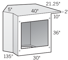
135° Radius Corner Cabinet w/10" Cantilever 30"D × 36"H OLPLSCC45
