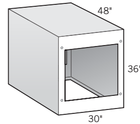
48" Cabinet 30"D x 36"H OLPLS0048
