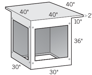
90° Corner Cabinet w/10" Cantilever on Two Sides 30"D x 30"L x 36"H OLPLSCHBC
