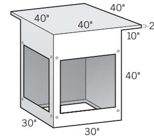
BAR-HEIGHT 90° Corner Cabinet w/10" Cantilever on Two Sides 30"D x 30"L x 40"H OLPLSBHBC
