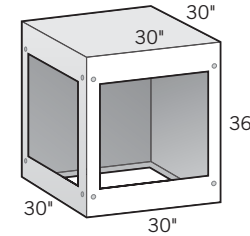
90° Corner Cabinet 30"D x 30"L x 36"H OLPLS00CN
