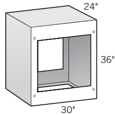
24" Cabinet 30"D x 36"H OLPLS0024
