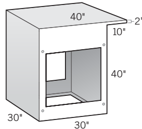
BAR-HEIGHT Cabinet w/10" Cantilever Backside 30"D x 30"L x 40"H OLPLSBHBS
